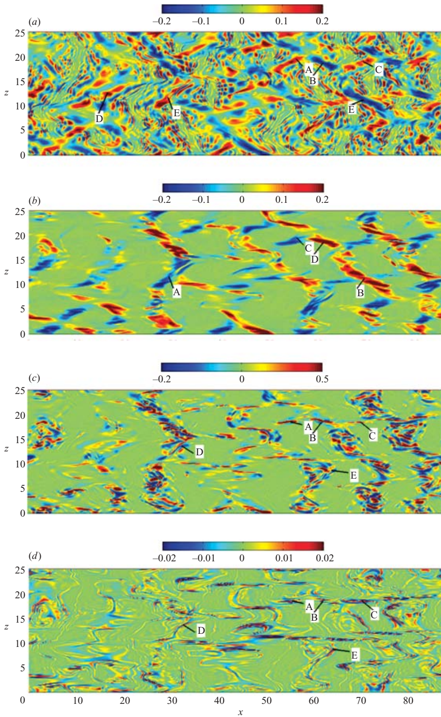
FIGURE 15. Different components of the vorticity transport equation for case A5, centre y -plane, t = 66.1 , (a) (1/\rho)g\partial\rho/\partial x , (b) \omega_z\partial v/\partial z , (c) \omega_z\partial w/\partial z , and (d) \nu\nabla^2\omega_z .
